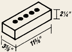
NORMAN
