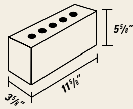
GIANT NORMAN
