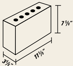
DOUBLE UTILITY
