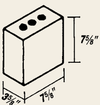
TRIPLE BRICK
