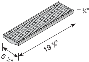
3/8" x 1 1/4" Grate Openings
