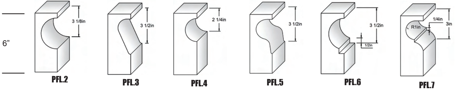
Sandstone
